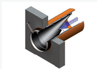
CHAMBER INSTALLATION
