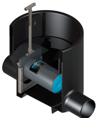
INLINE INSTALLATION
